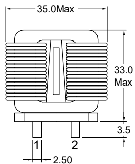
Orthographic view
