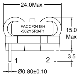
Orthographic view
