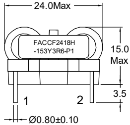
Orthographic view
