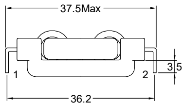
Orthographic view
