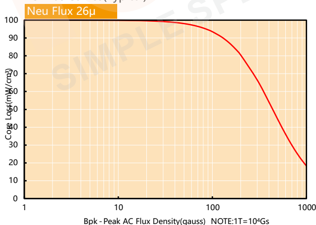
DC- Bias Curves(Typical)
