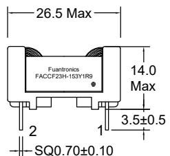
Orthographic view
