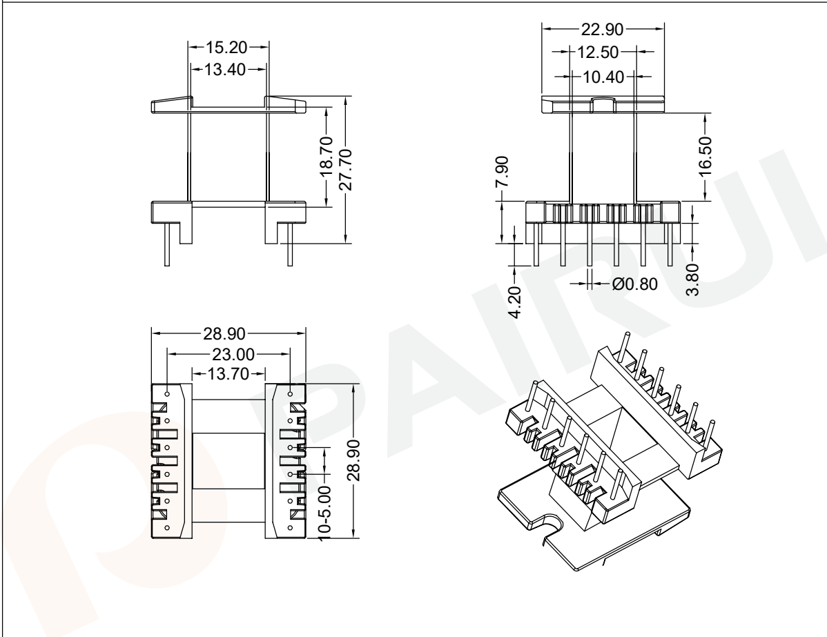
Winding data and area product for 12-pins EE33/14/13 coil former
