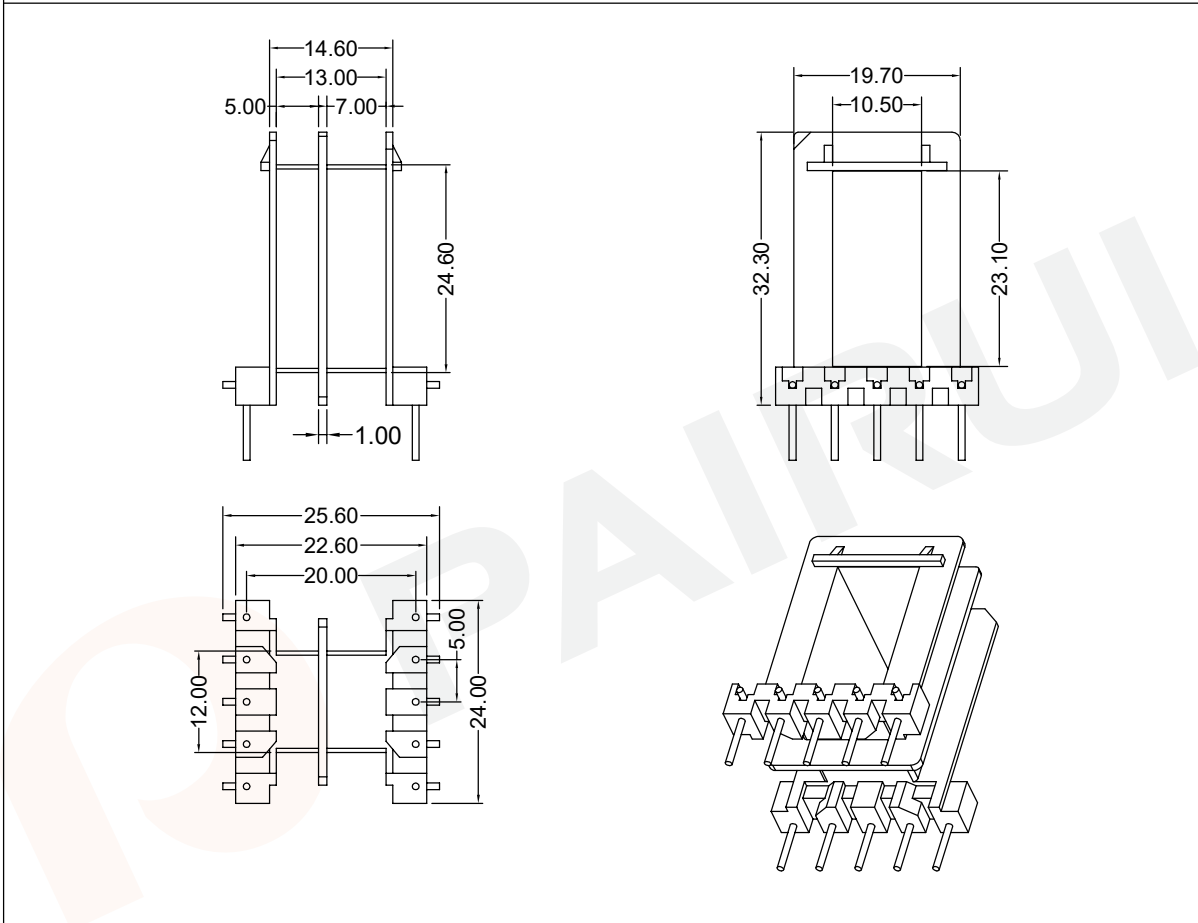
Winding data and area product for 10-pins EI30*23 coil former
