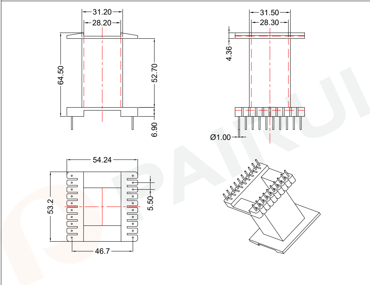
Winding data and area product for 20-pins EE85/44/26 coil former
